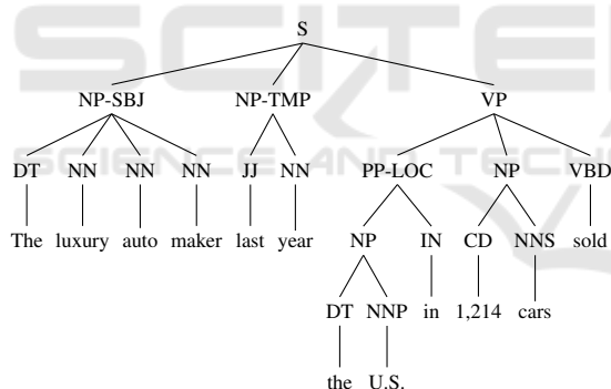
Figure 1: Phase-1-English tree for the parallel pair in Figure 2.
